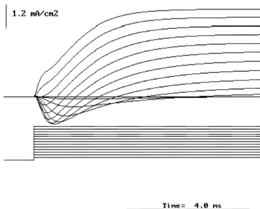
Figure 20. Currents in response to depolarizing pulses from -60 to 60 mV in increment of 10 mV from a holding potential of -70 mV.
