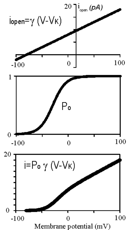
Figure 13. Top: the current through an open channel i , as a function of V . Middle: the open probability as a function of V for a long pulse (steady state). Bottom: the actual current.
