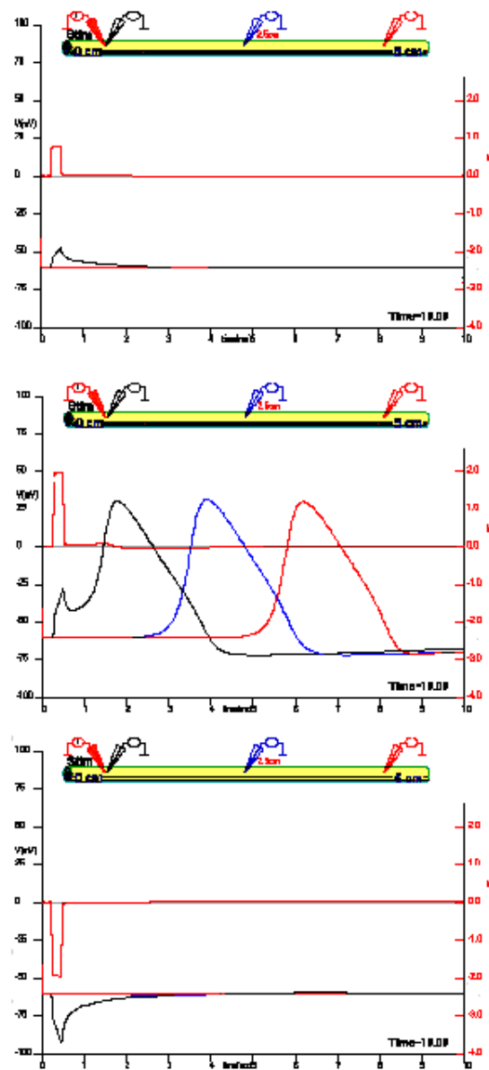
Figure 16. The response in three different locations of the axon to a variable stimulus at x=0 . Top panel: stimulus = 4 \mu\text{A} , middle panel: stimulus = 10 \mu\text{A} , bottom panel: stimulus = -10 \mu\text{A} .
