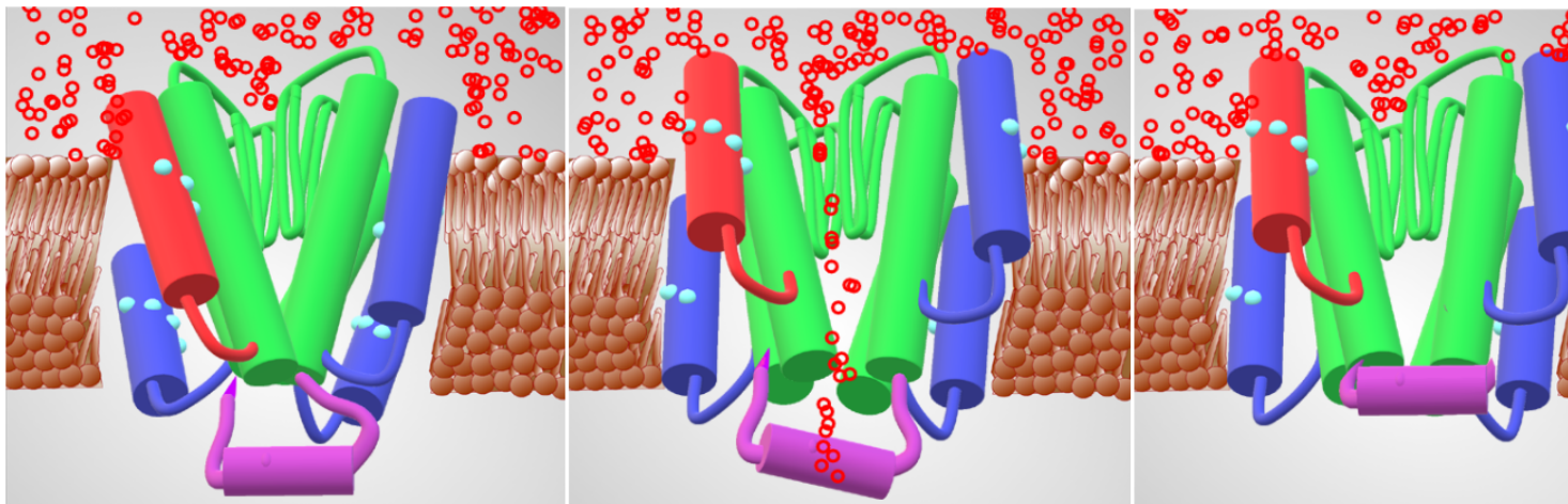
Plate 2. Schematic representation of the Na channel operation with sensors of Domains I, II and III in blue (fast) and sensor of Domain IV in red (slow). All four sensors couple to the bottom of S6 segments (in green) the gate. The channel conducts when Domains I, II and III are simultaneously active ( m^3 , according to the Hodgkin and Huxley formulation) but it also conducts when all four Domains are active. However the inactivating particle (violet) gets in position and blocks conduction after Domain IV goes into the active position.
