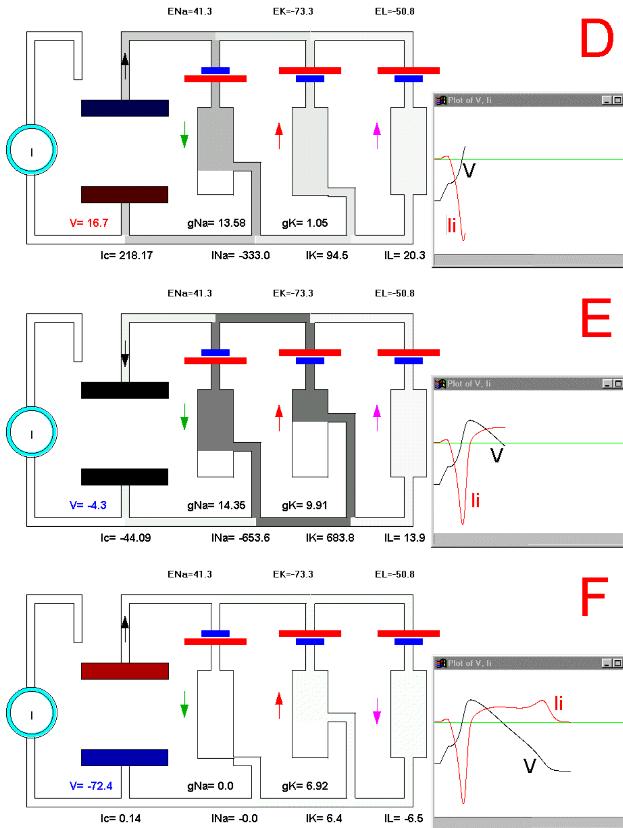
Plate 3. Currents and conductances in the equivalent circuit of the membrane during the action potential
