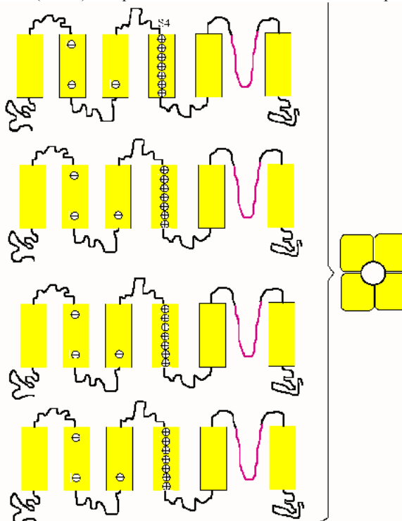
Figure 8. Each subunit of the K channel (left) has 6 transmembrane segments (S1 through S6). The S4 segment contains several basic residues. Between segment 5 and 6 there is a loop that, along with the S6 segment, lines the conduction pore. Four of these subunits are assembled in one functional K channel (right).
