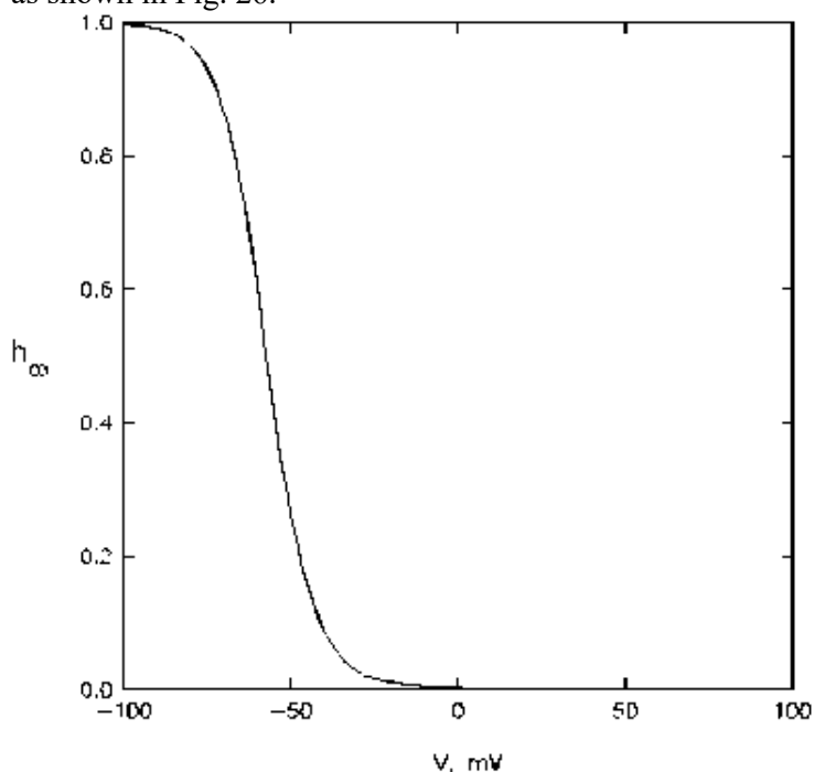
Figure 26. The voltage dependence of the effect of a long prepulse on the sodium current.
