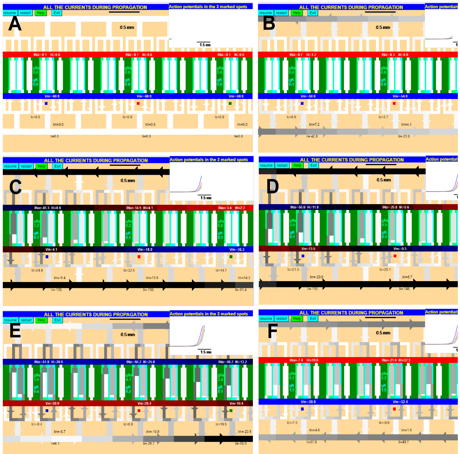
Figure 34. The currents underlying the propagation of the action potential simulated with several consecutive patches. The stimulating electrode is far away to the left of the two pictured patches color-coded red and blue. The time course of the action potential in each patch is shown above each panel and follows the color of the patch. The membrane potential in three of the patches is indicated in internal plate of the capacitor. The currents are shown in each branch and the values of the conductances are shown for the Na conductance (green) and K conductances (cyan) in three of the patches.
