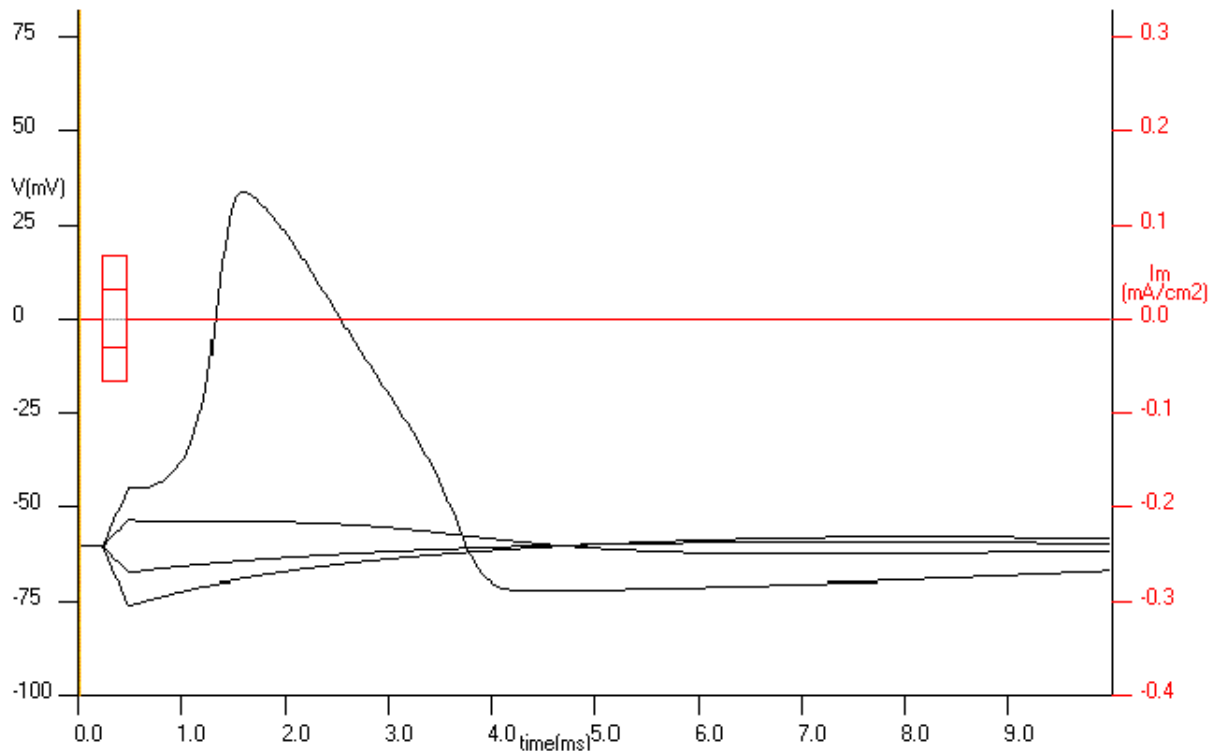
Figure 17. The response of an axon with an axial wire to stimuli of -10, -4.5, 4.5 and 10 uA . Only the stimulus of 10 uA elicited an action potential.
