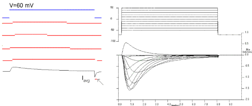
Figure 15. Single sodium channel records and average currents ( I_{avg} ) for pulses to -50, -35, 0, 30 and 60 mV starting and returning to -100 mV. Notice that the open probability is very small for pulses to -50 mV although the single channel current is the largest because there is a large driving force. The driving force reverses for a pulse to 60 mV because it is more positive than the Na reversal (equilibrium) potential. Occasionally, the channel does not inactivate even to the end of the pulse and a single channel event may be observed at the end of the pulse (see arrow for the pulse to 60 mV). The sum of these events produce the ionic "tail" observed at the end of the pulse. BOTTOM (right): family of Na currents for a series of depolarizations ranging from -50 to +60 mV, starting and ending at -70 mV.
